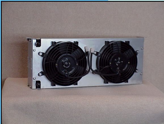
Remote Mt Condenser (735L x 270H x 160W) Twin fan, 4 row condenser , Available in Stainless steel or Powdercoated mild steel
